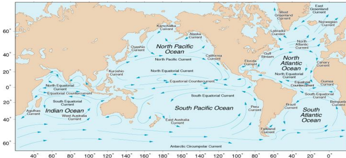
Figure 1.2a Major ocean surface currents including the five major gyres: Indian Ocean, North and South Atlantic, and North and South Pacific.
