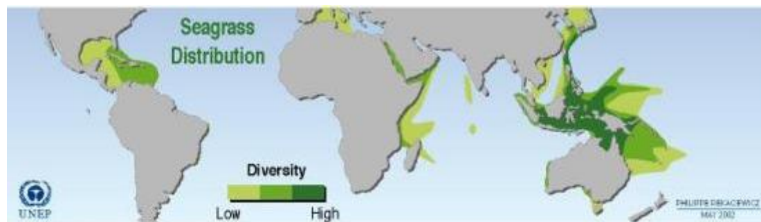
Figure 2.2a Global seagrass distribution and diversity
