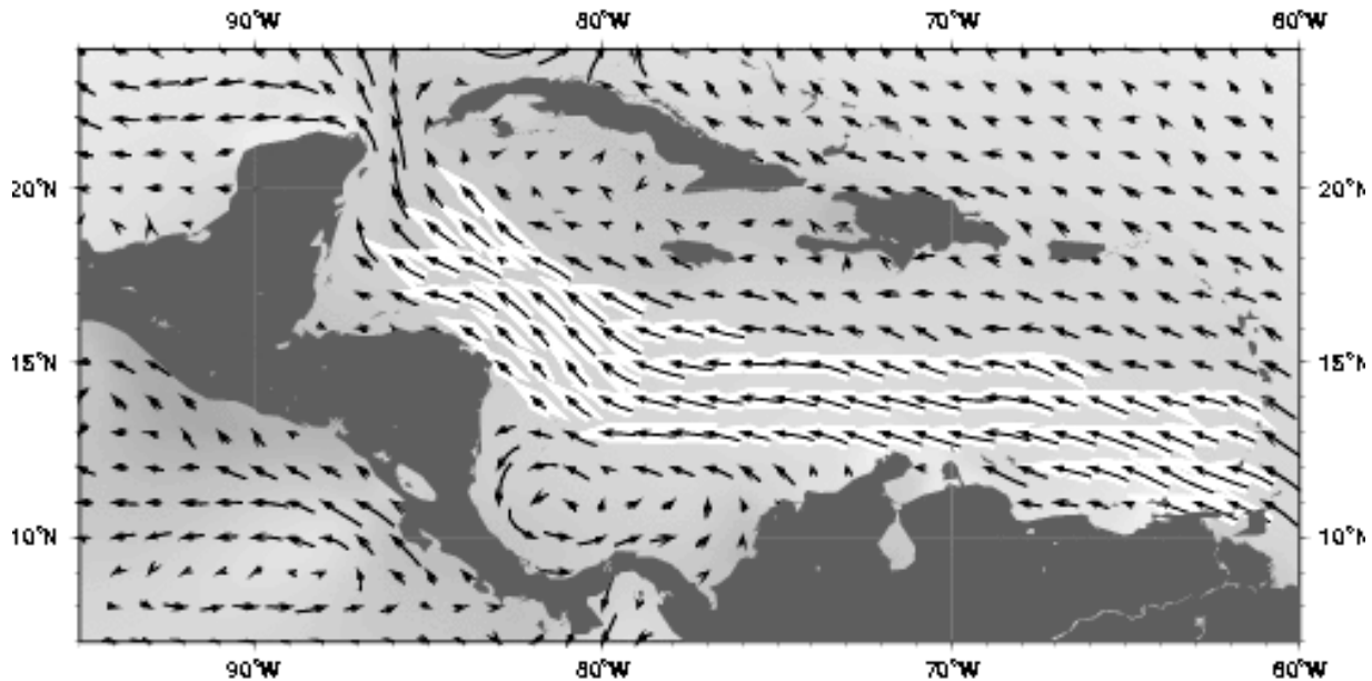
Figure 1.2b Surface Currents in the Caribbean Sea ( http://oceancurrents.rsmas.miami.edu/caribbean/caribbean.html )
